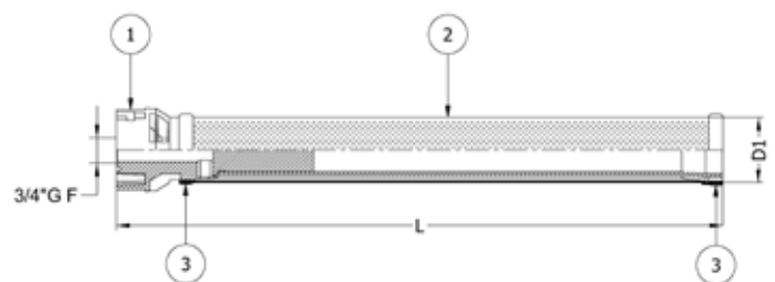
1 Holder 2 Membrane 3 Clamp
